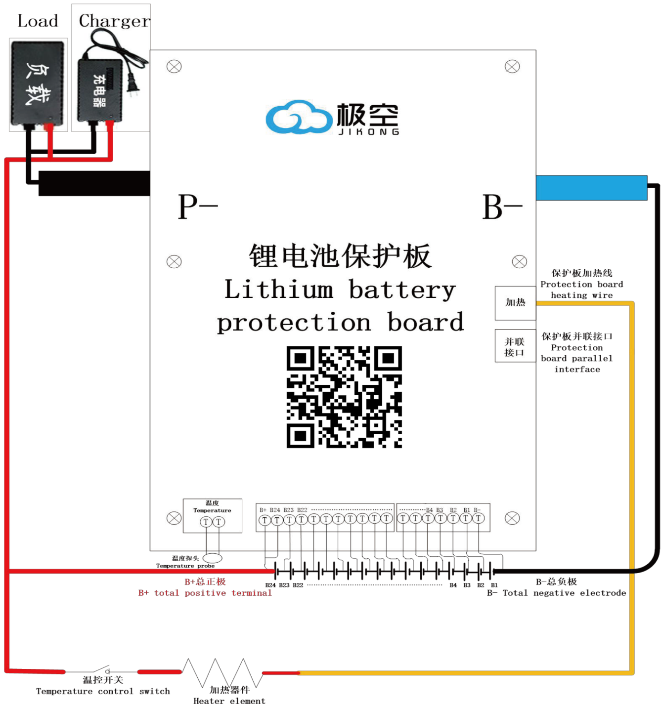
JK-BD4AxxS-6P/8P-24S接线图
